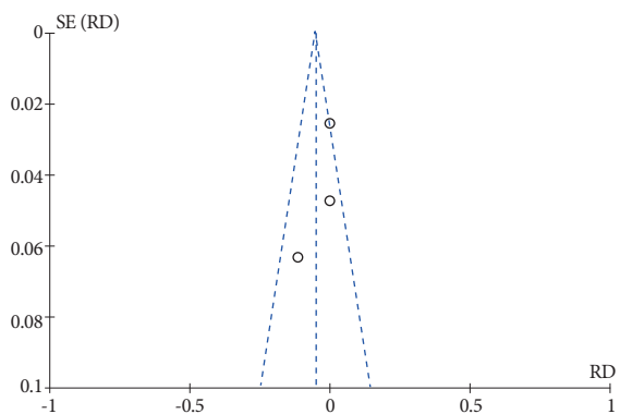
Supplementary Fig. 3. Funnel plot - Abdominal pain at 24 hours post-procedure. RD, the risk of difference; SE, standard error.
