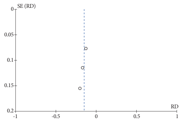
Supplementary Fig. 2. Funnel plot - Abdominal pain immediately post-procedure. RD, the risk of difference; SE, standard error.
