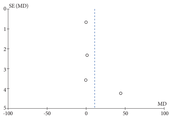
Supplementary Fig. 1. Funnel plot - Procedure time. MD, mean difference; SE, standard error.
